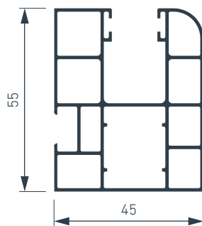
55x45 Comp. with Central 60x45 ■ 041001
