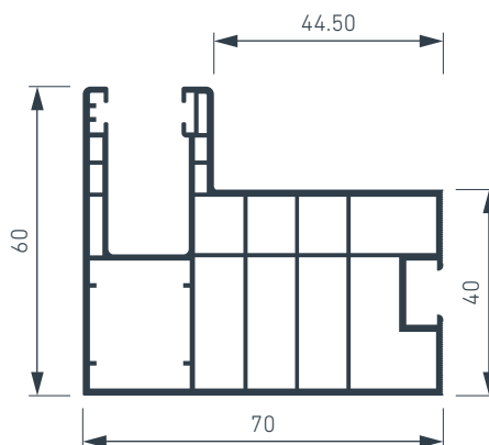
60x70 Compatible with Central 70x30 ■ 041011
