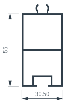
Fly Screen Ext. PVC 30x55
